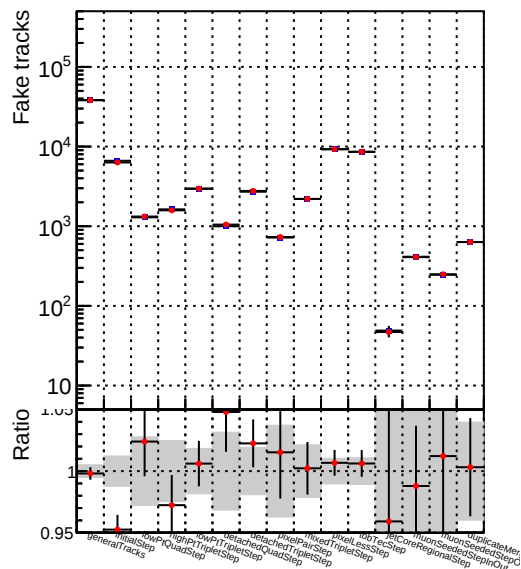
Number —●— DQM_TT_mkFit-DQM_original_newwindows
