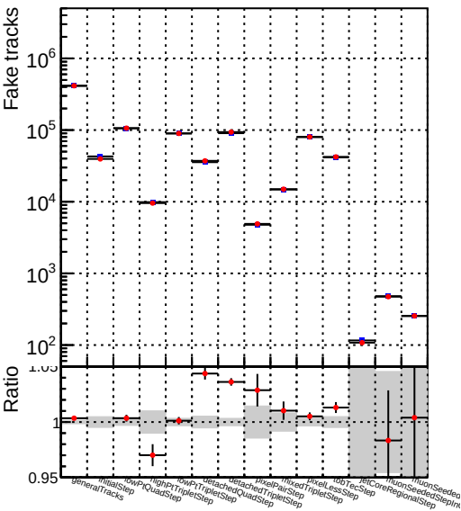
Number —●— DQM_TT_mkFit-DQM_original_newwindows
