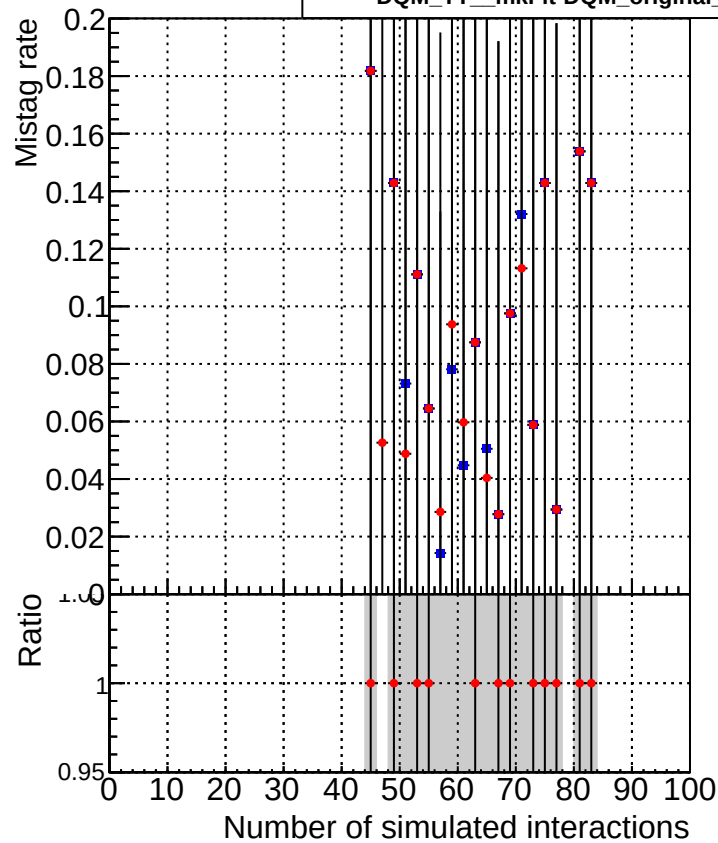
—■ DQM_TT_mkFit-DQM_original —● DQM_TT_mkFit-DQM_original_newwindows
