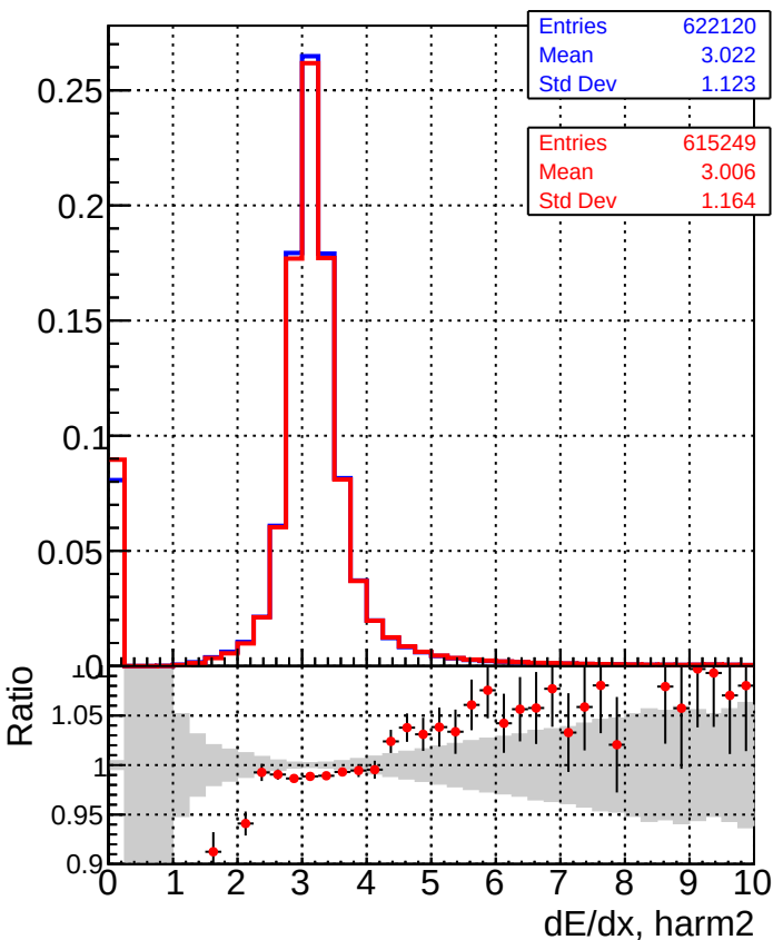
■ DQM_TT_mkFit-DQM_original ● DQM_TT_mkFit-DQM_original_newwindows
