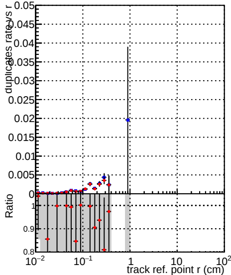
—•— DQM_TT_mkFit-DQM_original —•— DQM_TT_mkFit-DQM_original_newwindows
