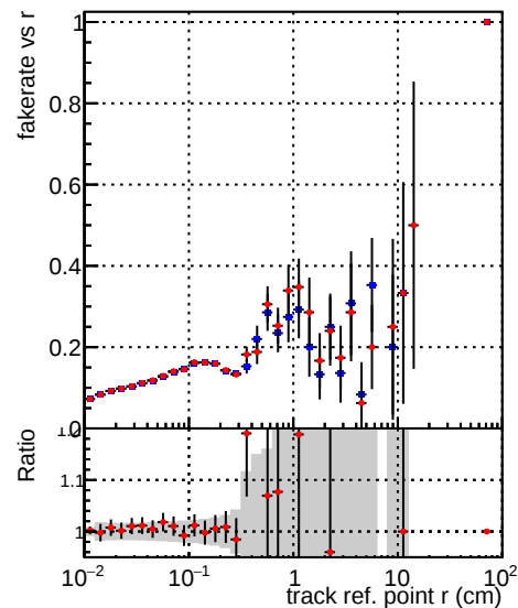
—•— DQM_TT_mkFit-DQM_original —•— DQM_TT_mkFit-DQM_original_newwindows
