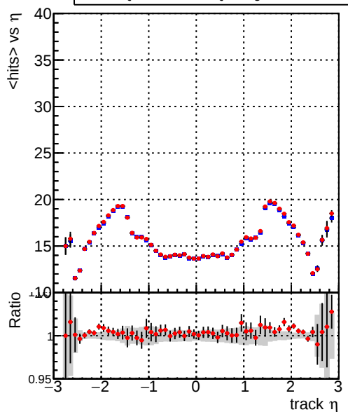
mean hits vs \eta — DQM_TT_mkFit-DQM_original — DQM_TT_mkFit-DQM_original_newwindows
