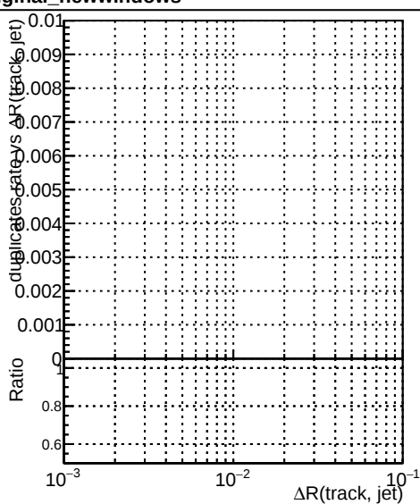
—•— DQM_TT_mkFit-DQM_original —•— DQM_TT_mkFit-DQM_original_newwindows
