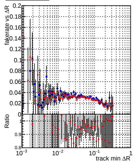
—•— DQM_TT_mkFit-DQM_original —•— DQM_TT_mkFit-DQM_original_newwindows
