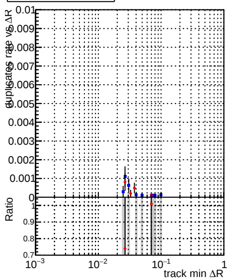
—•— DQM_TT_mkFit-DQM_original —•— DQM_TT_mkFit-DQM_original_newwindows
