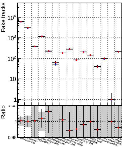
Number —●— DQM_TT_mkFit-DQM_original_newwindows
