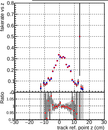
Fake rate vs vertpos —●— DQM_TT_mkFit-DQM_original —●— DQM_TT_mkFit-DQM_original_newwindows
