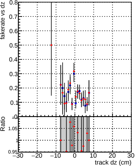
Fake rate vs dz Legend: DQM TT mkFit-DQM_original DQM TT mkFit-DQM_original newwindows
