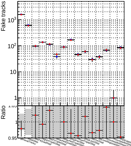
Number —●— DQM_TT_mkFit-DQM_original_newwindows
