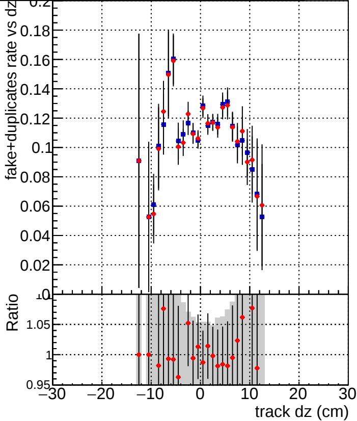
DQM_TT_mkFit-DQM_original DQM_TT_mkFit-DQM_original_newwindows
