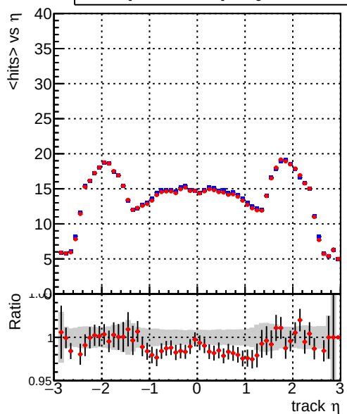
mean hits vs \eta Legend: — DQM_TT_mkFit-DQM_original — DQM_TT_mkFit-DQM_original_newwindows
