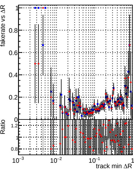
Fake rate vs \Delta R(\text{track, jet}) DQM_TT_mkFit-DQM_original DQM_TT_mkFit-DQM_original_newwindows
