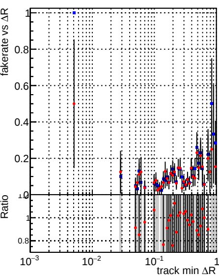
Fake rate vs \Delta R(\text{track, jet}) Legend: \blacksquare DQM_TT_mkFit-DQM_original \bullet DQM_TT_mkFit-DQM_original_newwindows
