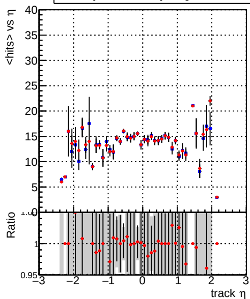
— DQM_TT_mkFit-DQM_original — DQM_TT_mkFit-DQM_original_newwindows mean hit
