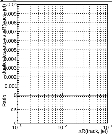
—●— DQM_TT_mkFit-DQM_original —●— DQM_TT_mkFit-DQM_original_newwindows
