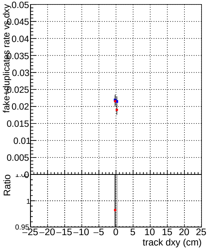
DQM_TT_mkFit-DQM_original DQM_TT_mkFit-DQM_original_newwindows
