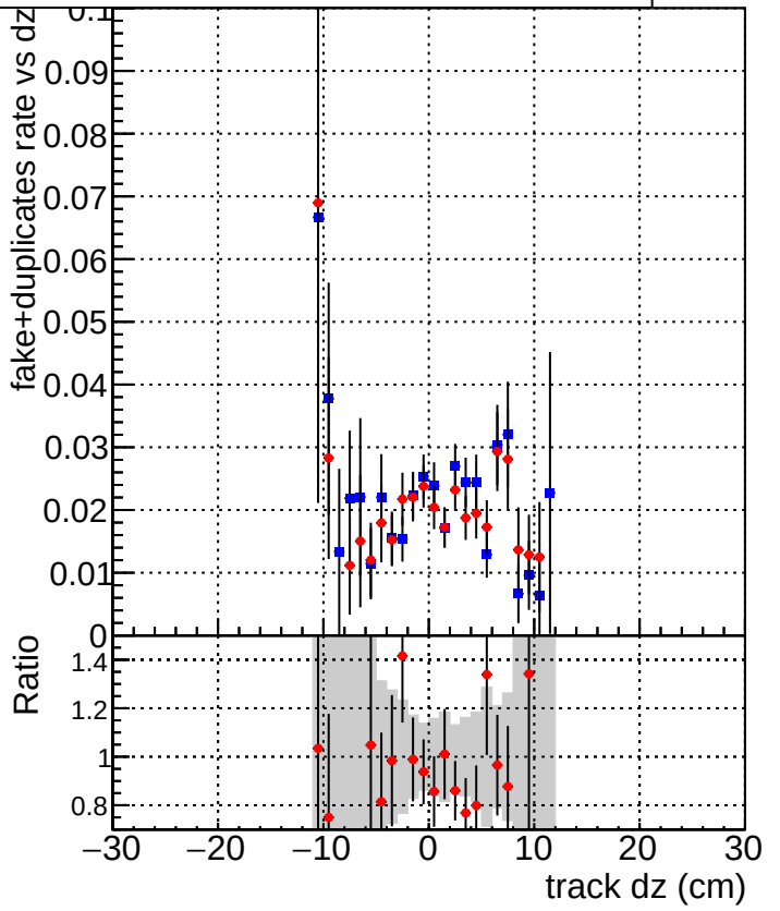
DQM_TT_mkFit-DQM_original DQM_TT_mkFit-DQM_original_newwindows
