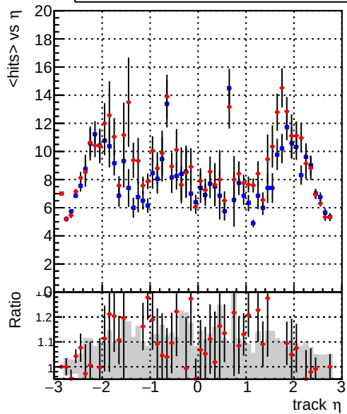
mean hit Legend: DQM_TT_mkFit-DQM_original (blue line with dots), DQM_TT_mkFit-DQM_original_newwindows (red line with dots)
