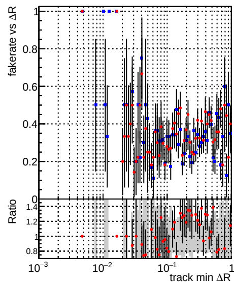
—•— DQM_TT_mkFit-DQM_original —•— DQM_TT_mkFit-DQM_original_newwindows
