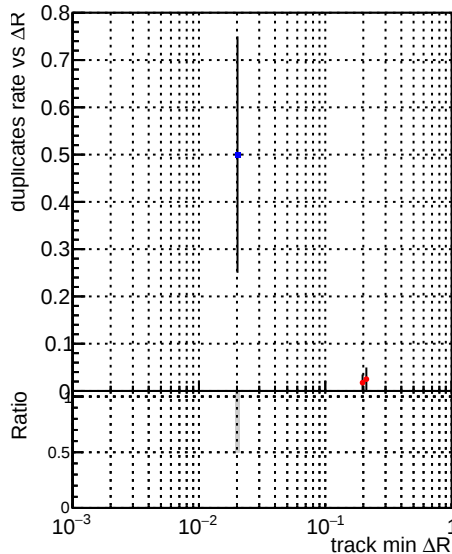
—•— DQM_TT_mkFit-DQM_original —•— DQM_TT_mkFit-DQM_original_newwindows
