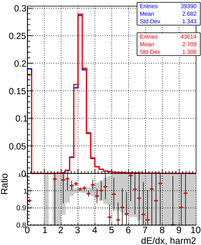
■ DQM_TT_mkFit-DQM_original ● DQM_TT_mkFit-DQM_original_newwindows
