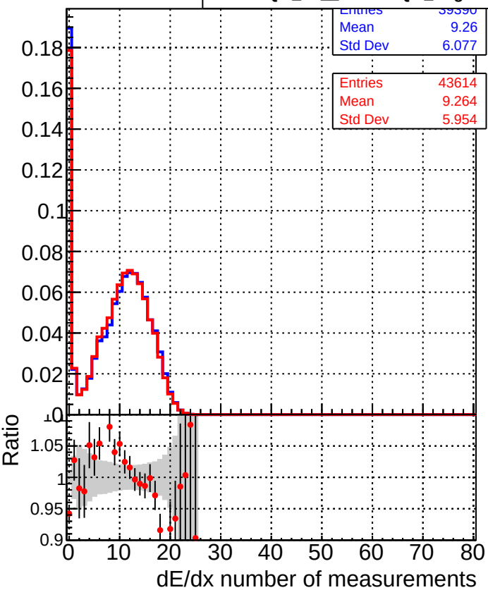
■ DQM_TT_mkFit-DQM_original ● DQM_TT_mkFit-DQM_original_newwindows
