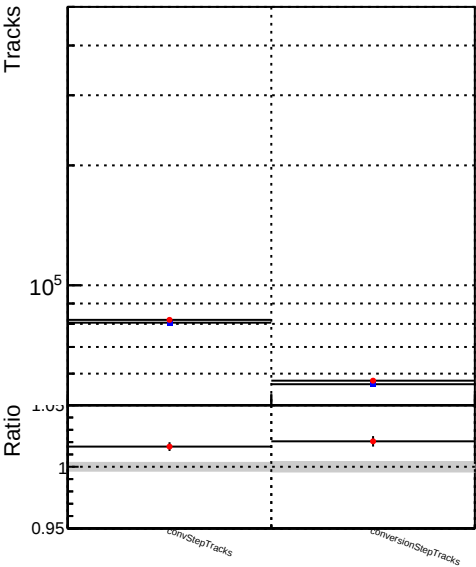
Number of tracks vs collection Legend: DQM_TT_mkFit-DQM_original DQM_TT_mkFit-DQM_original_newwindows
