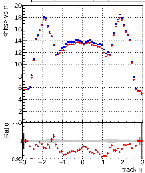
mean hits vs \eta Legend: DQM_TT_mkFit-DQM_original (blue line), DQM_TT_mkFit-DQM_original_newwindows (red line)
