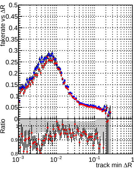
Fake rate vs \Delta R(\text{track, jet}) Legend: —●— DQM_TT_mkFit-DQM_original —●— DQM_TT_mkFit-DQM_original_newwindows
