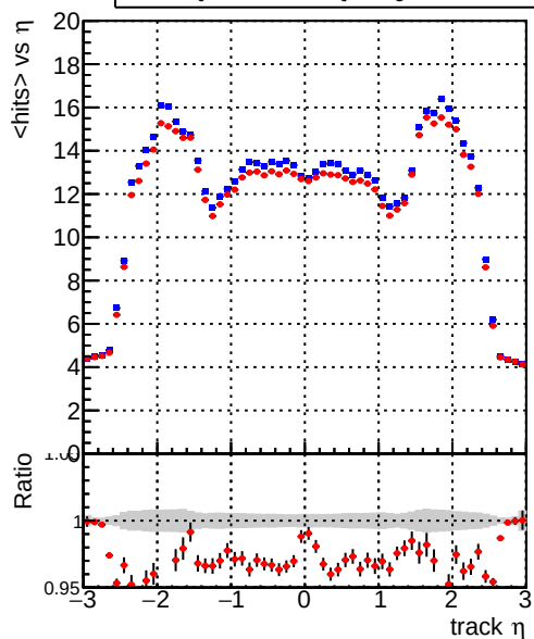
mean hits Legend: DQM_TT_mkFit-DQM_original (blue line), DQM_TT_mkFit-DQM_original_newwindows (red line)
