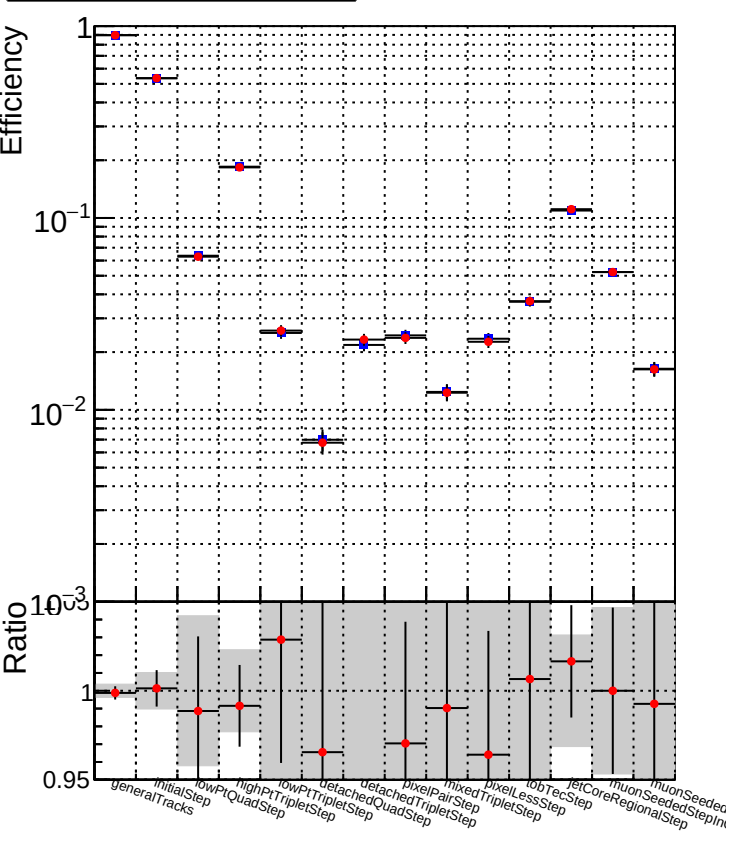
DQM_TT_mkFit-DQM_original DQM_TT_mkFit-DQM_original_newwindows
