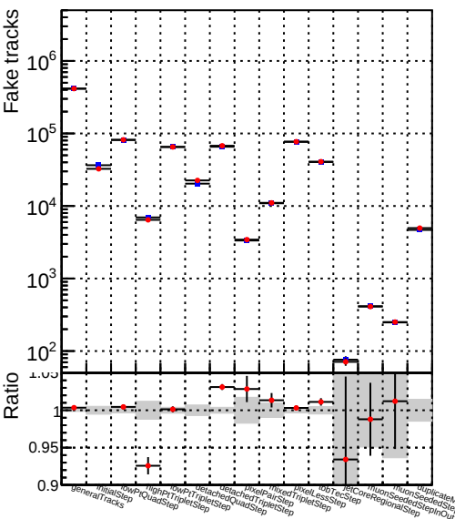
Number —●— DQM_TT_mkFit-DQM_original_newwindows
