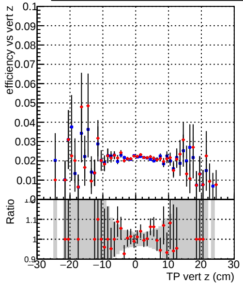
Efficiency vs vert z — DQM_TT_mkFit-DQM_original — DQM_TT_mkFit-DQM_original_newwindows
