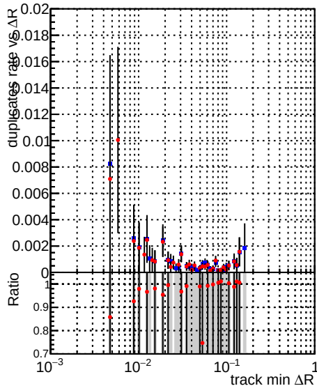
—•— DQM_TT_mkFit-DQM_original —•— DQM_TT_mkFit-DQM_original_newwindows
