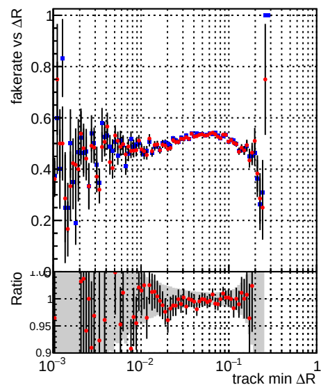
—•— DQM_TT_mkFit-DQM_original —•— DQM_TT_mkFit-DQM_original_newwindows
