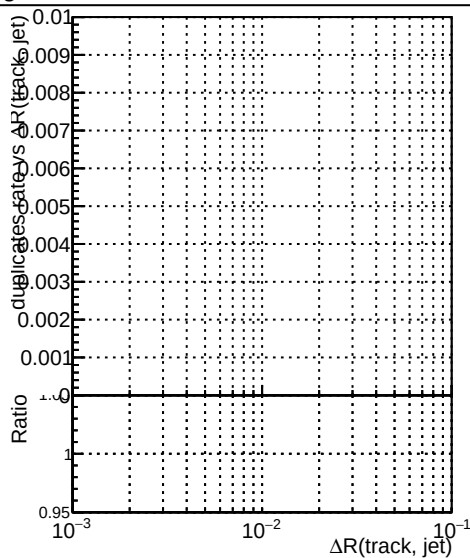
—•— DQM_TT_mkFit-DQM_original —•— DQM_TT_mkFit-DQM_original_newwindows
