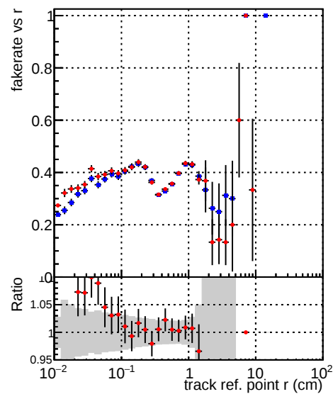
—■— DQM_TT_mkFit-DQM_original —●— DQM_TT_mkFit-DQM_original_newwindows
