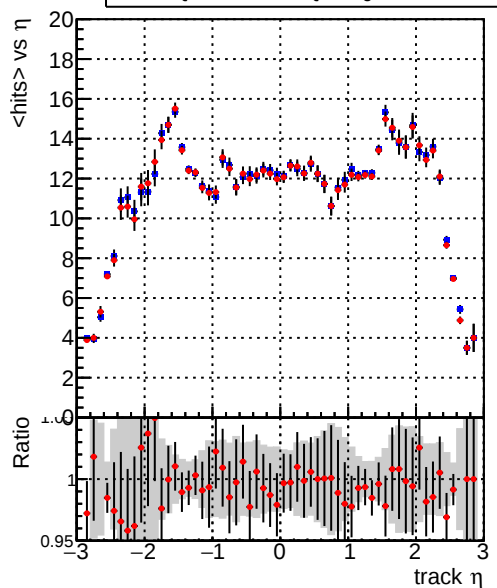
— DQM_TT_mkFit-DQM_original — DQM_TT_mkFit-DQM_original_newwindows mean hits
