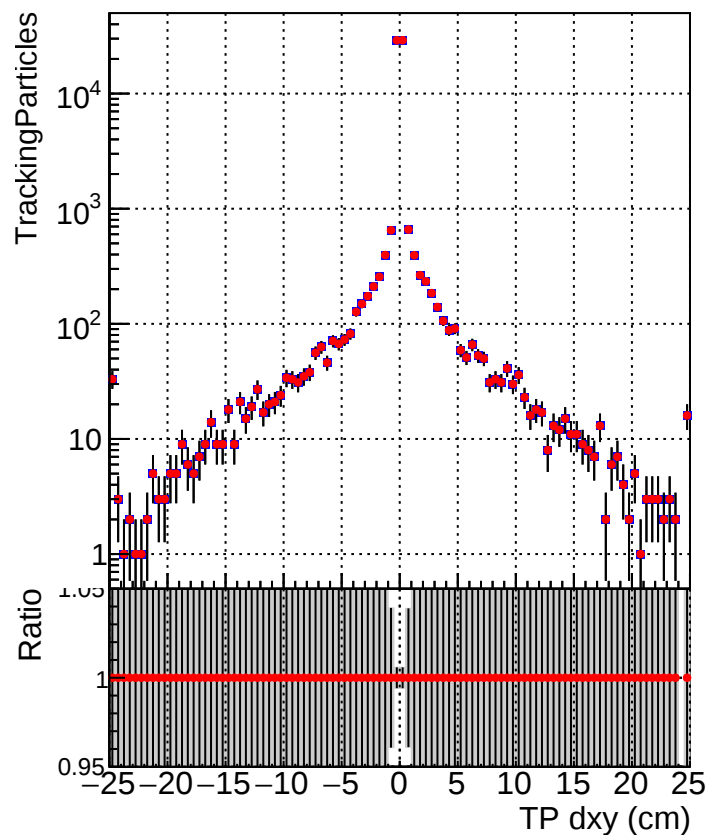
■ DQM_TT_mkFit-DQM_original ■ DQM_TT_mkFit-DQM_original_newwindows
