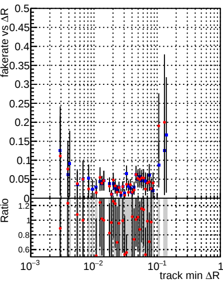
Fake rate vs \Delta R(\text{track}, \text{jet}) Legend: —■— DQM_TT_mkFit-DQM_original —●— DQM_TT_mkFit-DQM_original_newwindows
