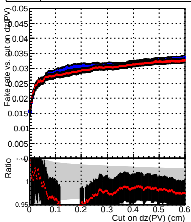
Fake rate — DQM_TT_mkFit-DQM_original_newwindows
