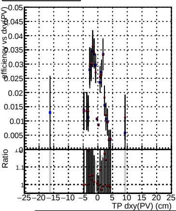
Efficiency vs Dxy(PV) Legend: DQM_V0001_R000000001_Global_mkFitOLD_RECO DQM_V0001_R000000001_Global_mkFit100_RECO DQM_V0001_R000000001_Global_mkFit100tobtec_RECO
