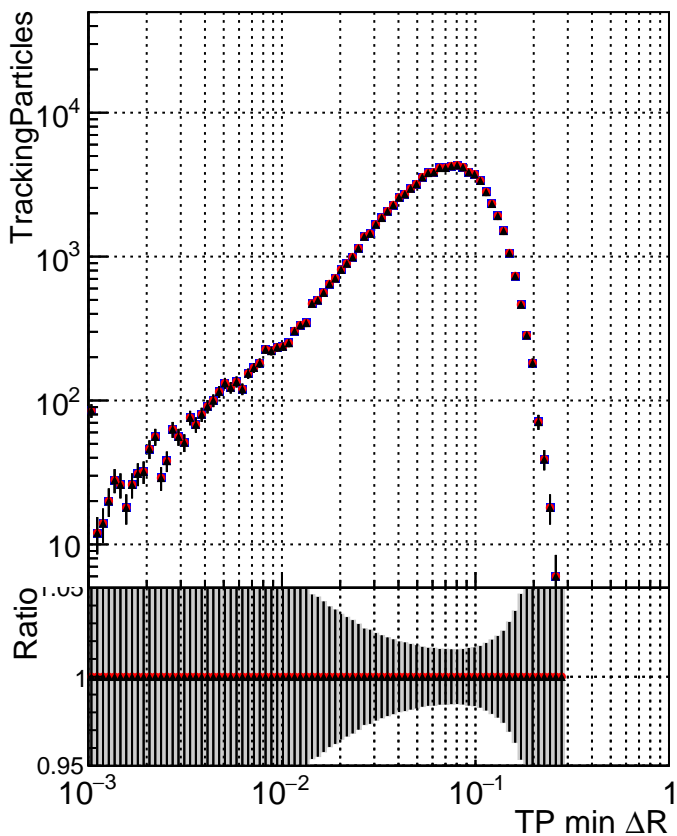
N of simulated tracks vs ΔR(TP, jet)
