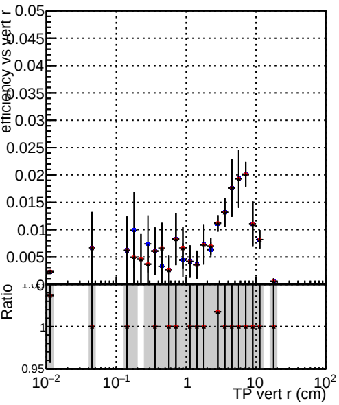
Efficiency vs vertpos Blue circle DQM_V0001_R000000001_Global_mkFitOLD_RECO Red circle DQM_V0001_R000000001_Global_mkFit100_RECO Black circle DQM_V0001_R000000001_Global_mkFit100tobtec_RECO
