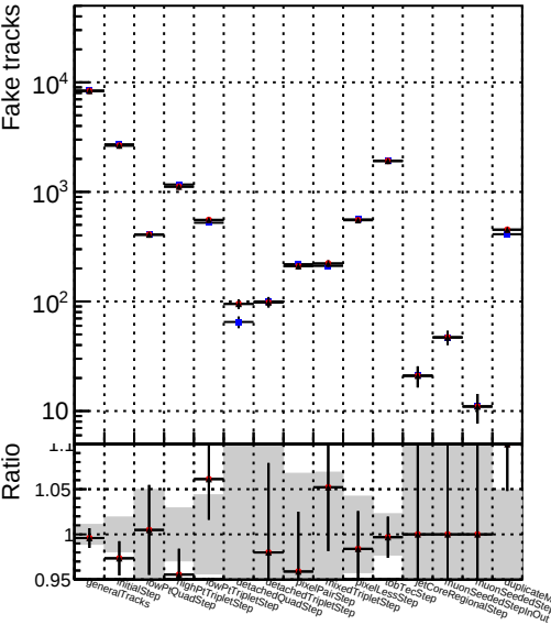
Number ● DQM_V0001_R0000000001_Global_mkFit100_RECO ▲ DQM_V0001_R0000000001_Global_mkFit100tobtec_RECO
