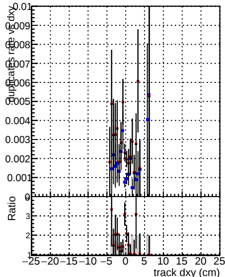
— DOM V0001 RECO — DOM V0001 RECO — Global fit OLD RECO — Global fit OLD RECO — Global fit OLD RECO — Global fit OLD RECO
