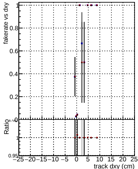
Legend for all plots: DOM V0001 RECO (Blue dots) DOM V0001 RECO (Red dots) Global fitOLD RECO (Black line) Global fit100 RECO (Black line) Global fit100robtec RECO (Black line)
