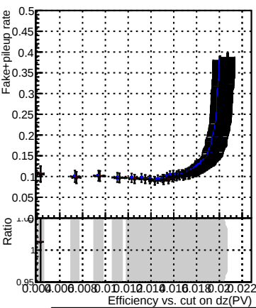
Legend: DQM_V0001_R000000001_Global_mkFitOLD_RECO DQM_V0001_R000000001_Global_mkFit100_RECO DQM_V0001_R000000001_Global_mkFit100tobtec_RECO
