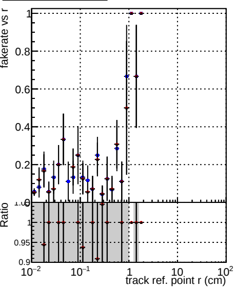
DQM_V0001_R000000001 Global mkFitOLD RECO DQM_V0001_R000000001 Global mkFit100 RECO DQM_V0001_R000000001 Global mkFit100tobtec RECO
