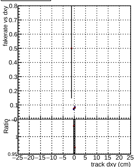
Fake rate vs d DOM V0001 R0000000001 Global mkFitOLD RECO DOM V0001 R0000000001 Global mkFit100 RECO DOM V0001 R0000000001 Global mkFit100tofbtec RECO
