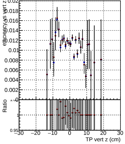
Efficiency vs. TP vert z (cm) —●— DQM_V0001_R0000000001_Global_mkFitOLD_RECO —●— DQM_V0001_R0000000001_Global_mkFit100_RECO —●— DQM_V0001_R0000000001_Global_mkFit100tobtec_RECO
