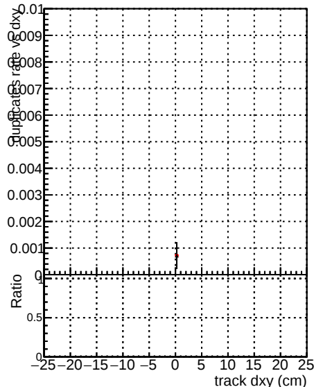
Legend for Fake rate vs dxy, Duplicates Rate vs Dxy, and Pileup rate vs dxy: DOM V0001 RECO (Blue circles) DOM V0001 RECO (Red circles) Global mkFitOLD RECO (Black circles) Global mkFit100 RECO (Black circles) Global mkFit100robtec RECO (Black circles)
