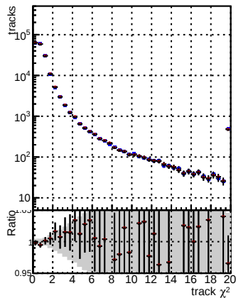
N of reco track vs. s Legend DOM V0001 R0000000001 Global mkFitOLD RECO Blue dot DOM V0001 R0000000001 Global mkFitOLD RECO Red dot DOM V0001 R0000000001 Global mkFit100 RECO Black dot DOM V0001 R0000000001 Global mkFit100 RECO
