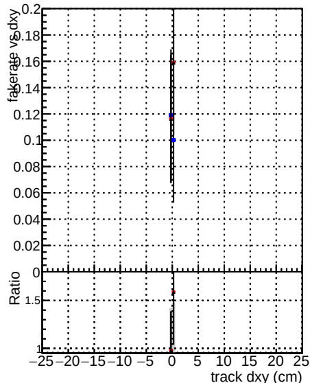
DOM V0001 R0000000001 Global mkFitOLD RECO Fake rate vs d Blue line with dots Red line with dots Black line with dots Duplicates Rate vs Dxy Blue line with dots Red line with dots Black line with dots Pileup rate vs dxy Blue line with dots Red line with dots Black line with dots
