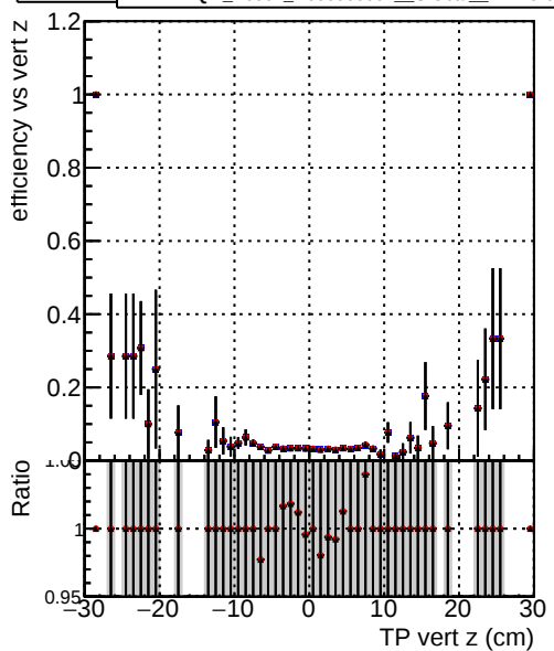
Efficiency vs. sim PV z —●— DQM_V0001_R0000000001_Global_mkFitOLD_RECO —●— DQM_V0001_R0000000001_Global_mkFit100_RECO —●— DQM_V0001_R0000000001_Global_mkFit100tobtec_RECO
