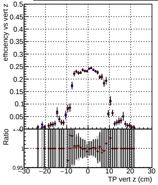
Efficiency vs vertpos Blue line with error bars DQM_V0001_R000000001_Global_mkFitOLD_RECO Red line with error bars DQM_V0001_R000000001_Global_mkFit100_RECO Black line with error bars DQM_V0001_R000000001_Global_mkFit100tobtec_RECO
