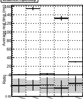
detachedTripletStep
