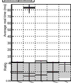
jetCoreRegionalStep
