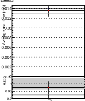
Other
