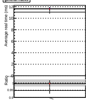
generalTracks
